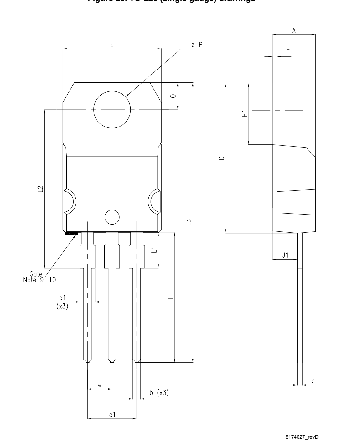
Figure 13. TO-220 (single gauge) drawings
